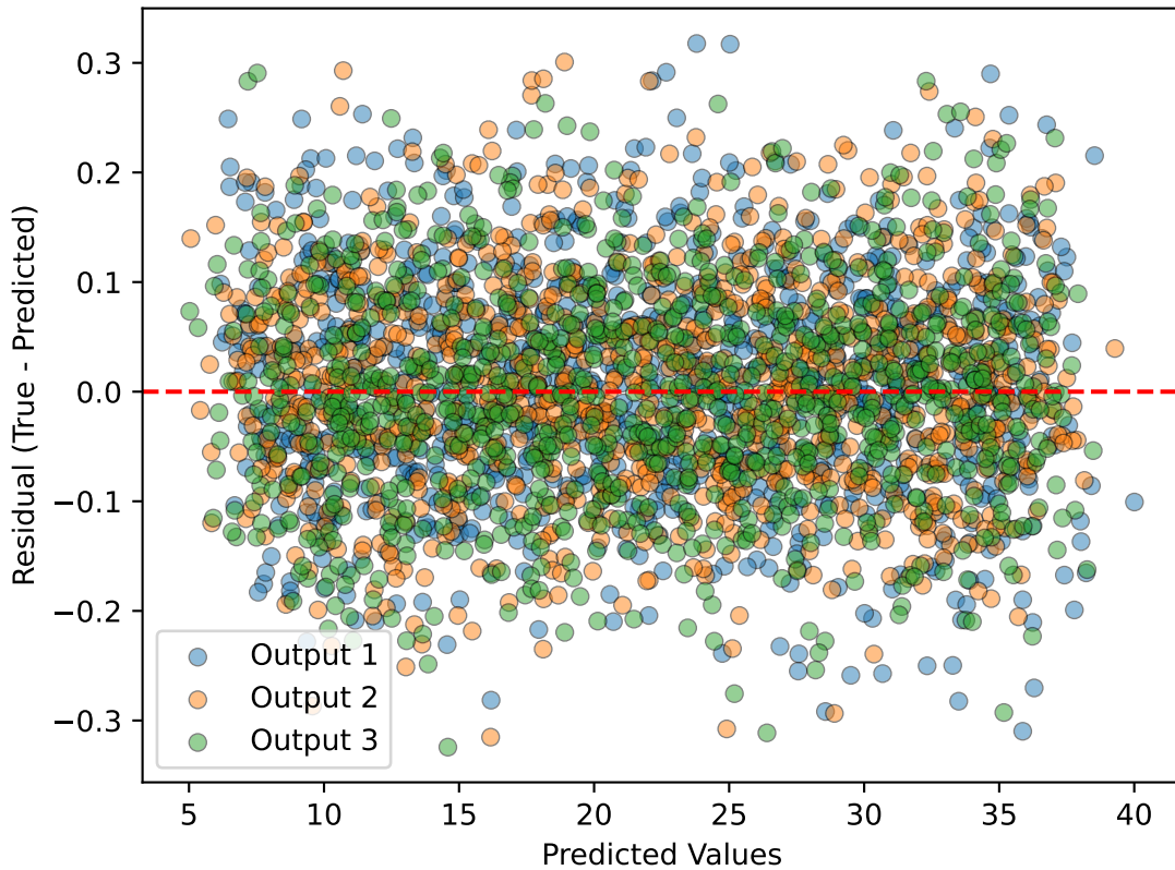
Linear Regression Data: Residuals vs. Predicted Values
