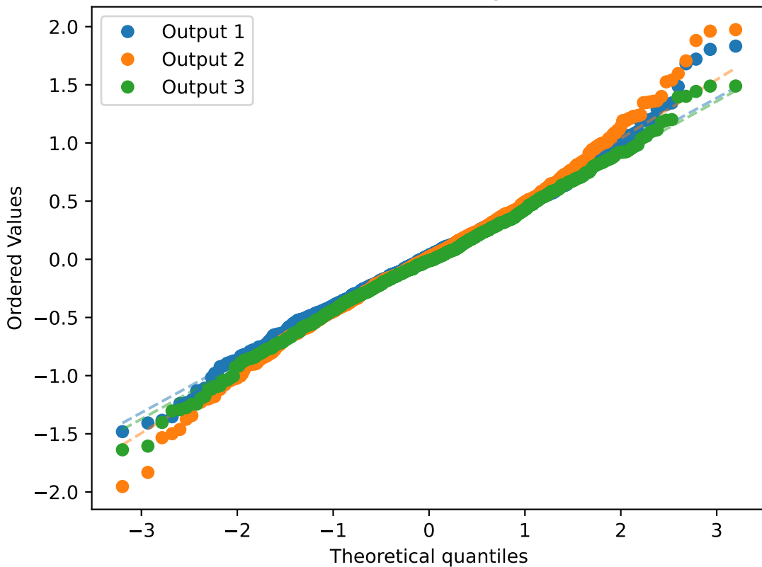
Q-Q Plot: Linear Regression
