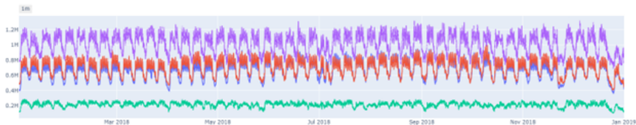
Figure 57. Annual industrial electrical profiles for Met Ed (blue), Penelc (red), Penn Power (green), and West Penn Power (purple).
