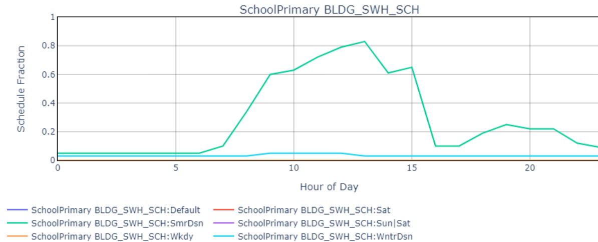
Figure 77. SWH heating usage schedule for primary school.
