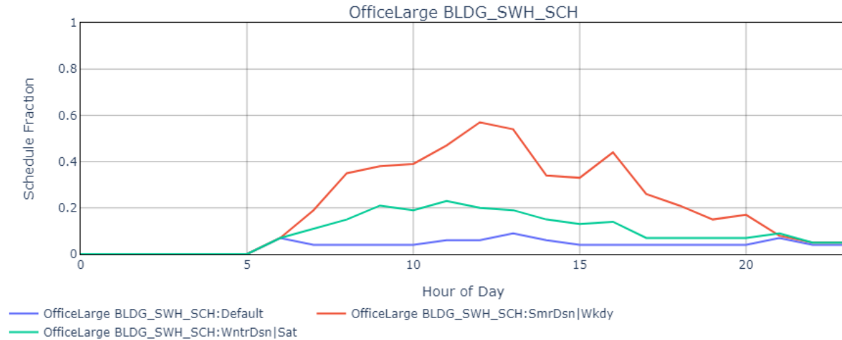
Figure 73. SWH heating usage schedule for large office.
