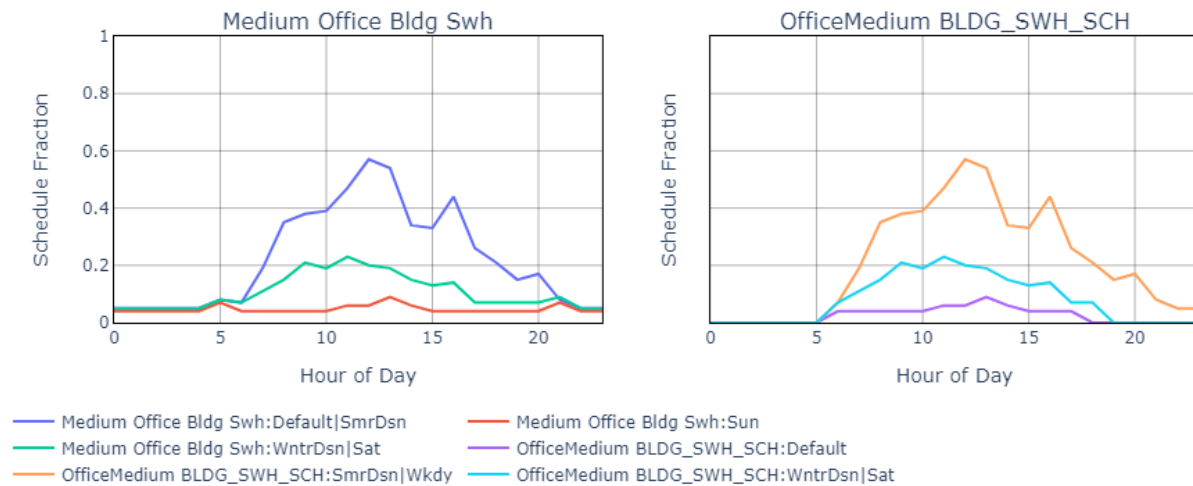
Figure 74. SWH heating usage schedule for medium office.
