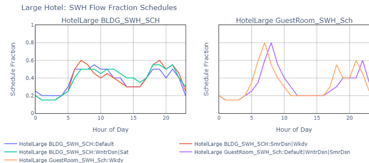
Figure 72. SWH heating usage schedule for large hotel.
