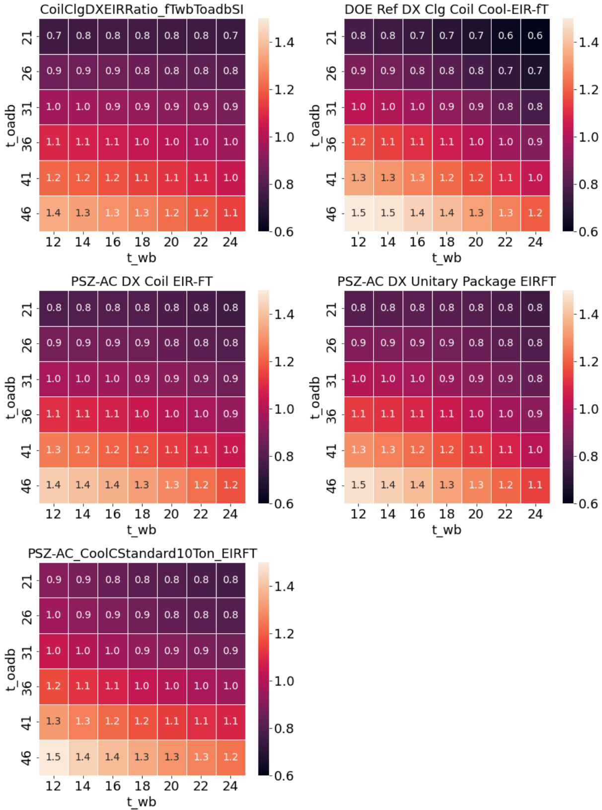
Figure 104. DX cooling energy input ratio as a function of temperature performance curves. Independent variables are outdoor air dry bulb temperature (y-axis, degrees Celsius) and wet bulb temperature entering the cooling coil (x-axis, degrees Celsius).
