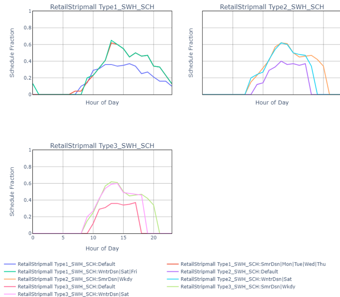
Figure 82. SWH heating usage schedule for strip mall.
