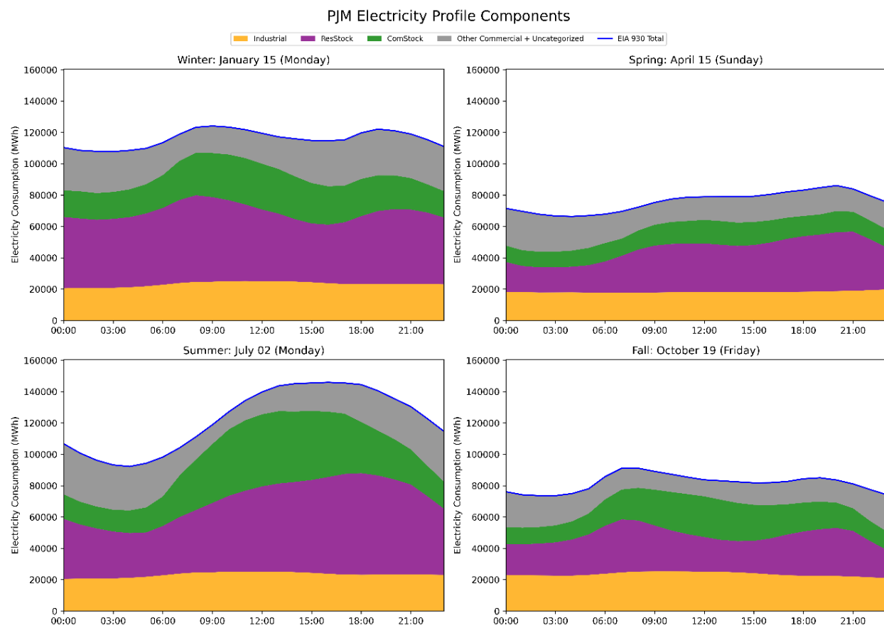
Figure 61. PJM Electricity Profile Components
