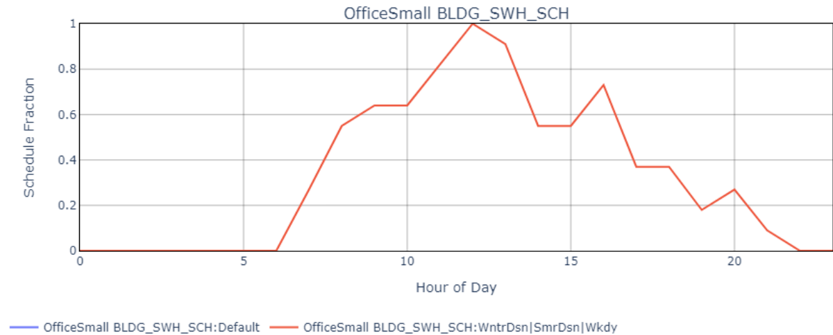
Figure 75. SWH heating usage schedule for small offices.
