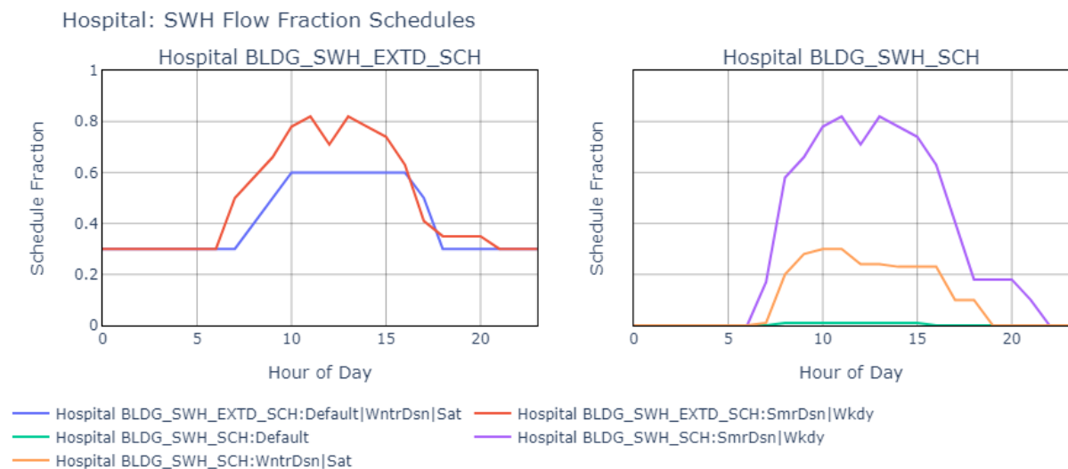
Figure 71. SWH heating usage schedule for hospitals.
