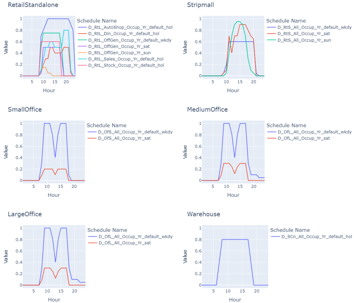
Figure 69. California base occupancy schedules for retail, office, and warehouse ComStock building types.
