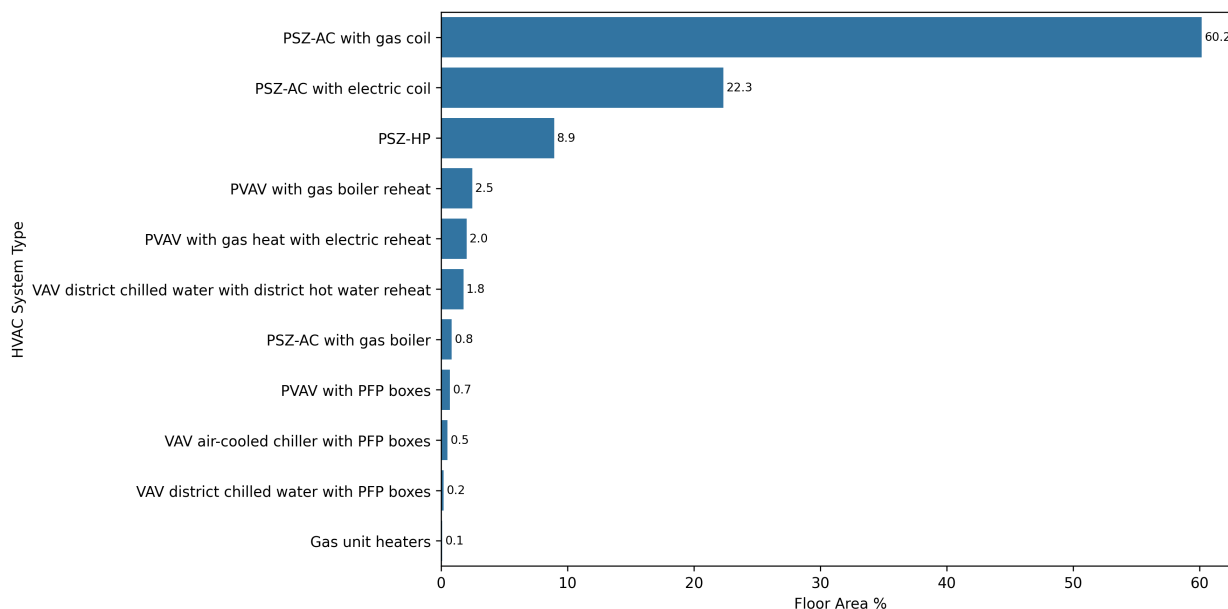
Figure 73. Prevalence of ComStock HVAC system types by total stock floor area; all building types.
