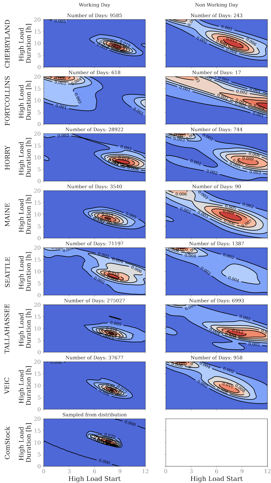
Figure 57. Distribution of small office hours of operations extracted from AML data (from seven utilities), by utility and day type, and compared to ComStock before updates. This figure shows how the hours of operation (start time and duration of the high load period) are influenced by utility region (all seasons are combined in this plot).
