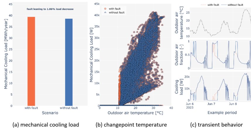
Figure 51. Economizer incorrect changeover temperature setting fault impact on simulation results.
