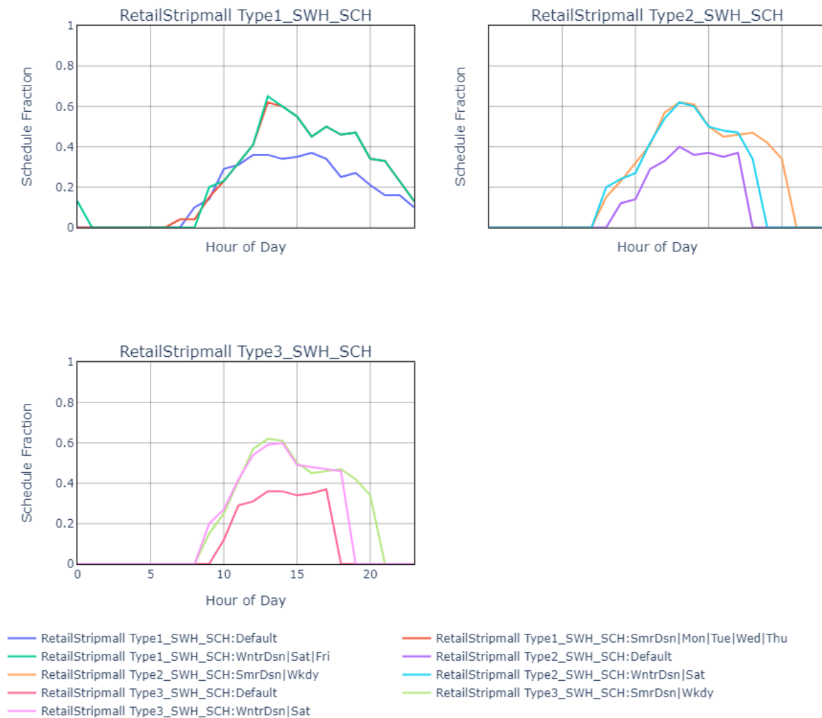
Figure 72. SWH heating usage schedule for strip mall.
