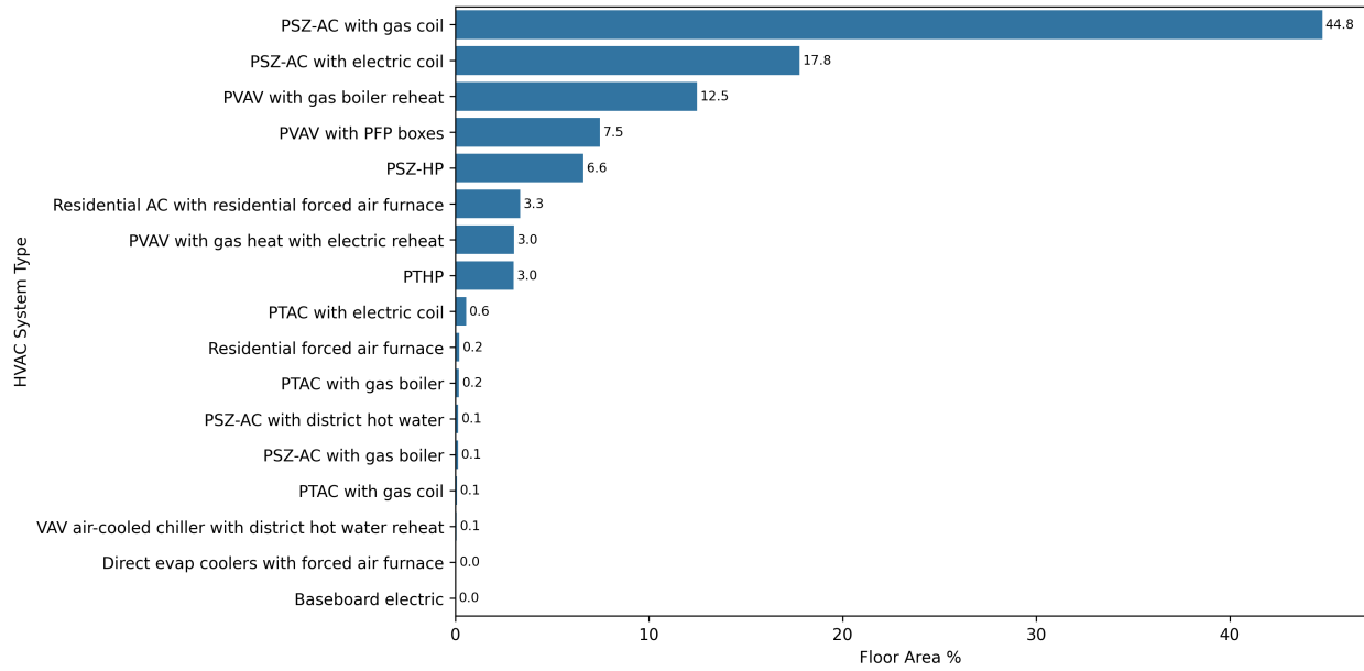
Figure 83. Prevalence of ComStock HVAC system types by total stock floor area; retail.
