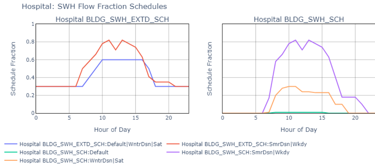
Figure 61. SWH heating usage schedule for hospitals.
