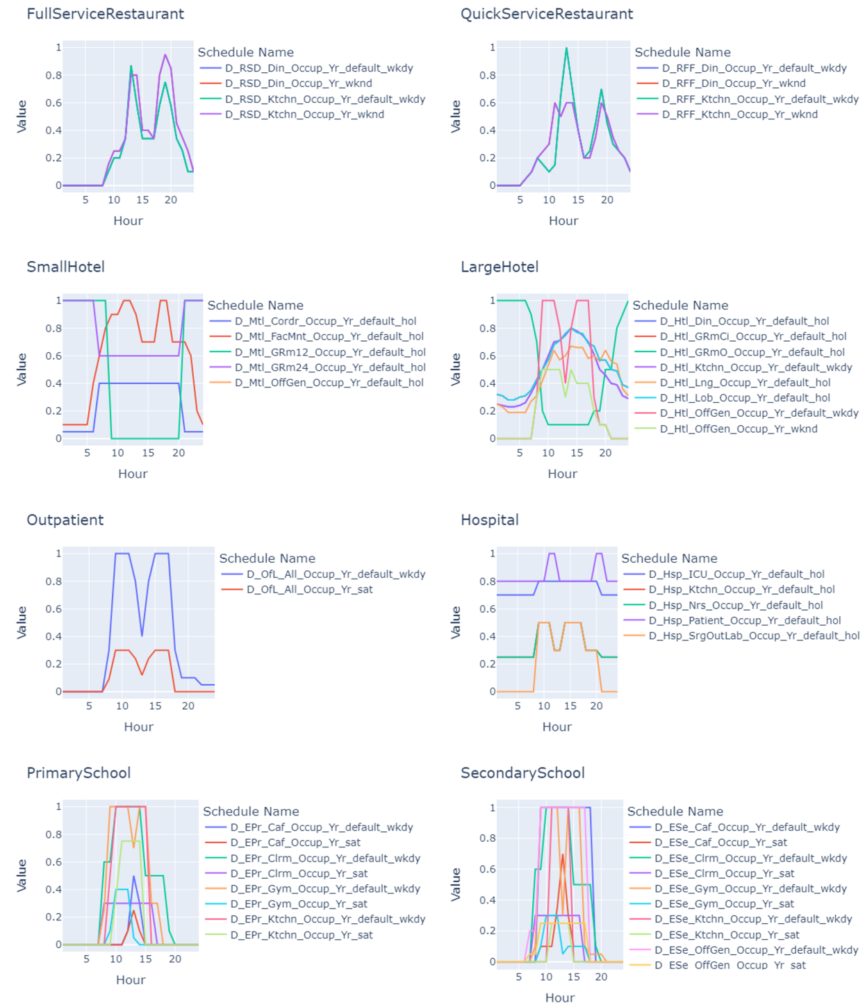
Figure 58. California base occupancy schedules for food service, lodging, healthcare, and education ComStock building types.
