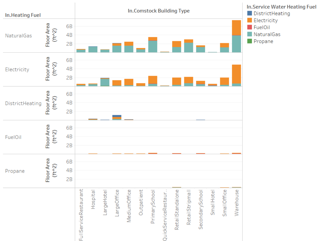
Figure 37. Floor area served by each service water heating fuel by space heating fuel and building type.
