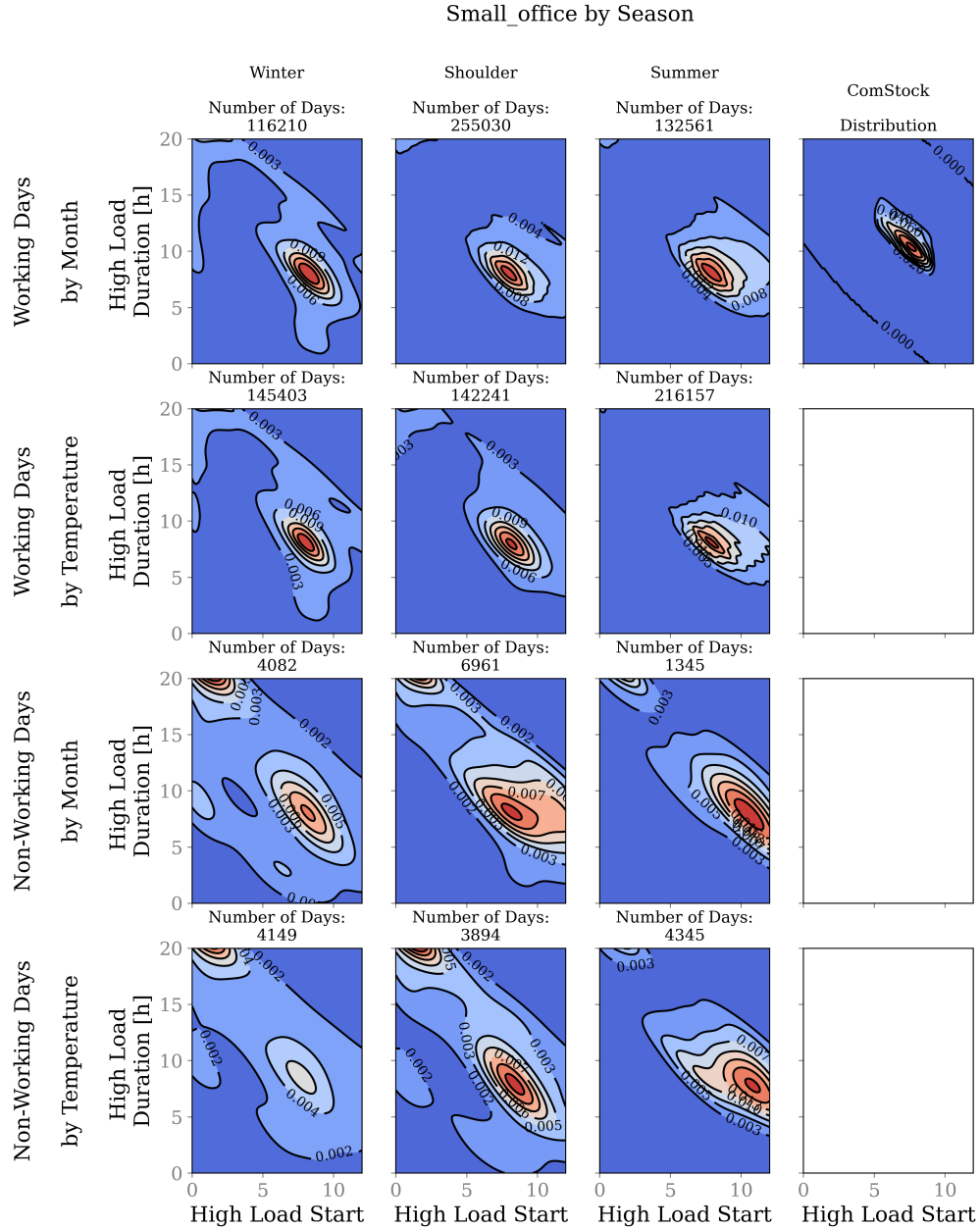
Figure 56. Distribution of small office hours of operations extracted from AML data (from seven utilities), by day type and season, and compared to ComStock before updates. This figure shows how the hours of operation (start time and duration of the high load period) are influenced by season (all utilities are combined in this plot).
