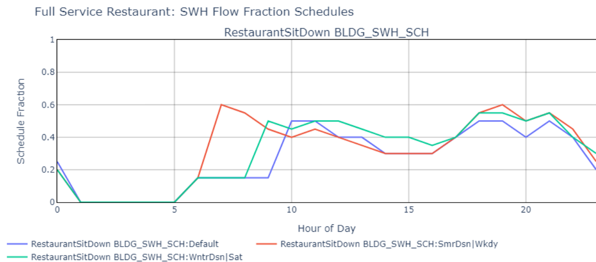
Figure 60. SWH heating usage schedule for full service restaurants.
