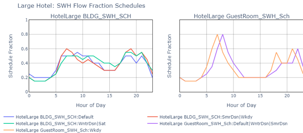
Figure 62. SWH heating usage schedule for large hotel.
