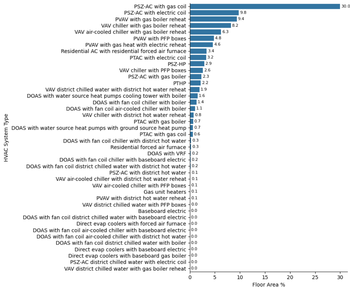
Figure 73. Prevalence of ComStock HVAC system types by total stock floor area; all building types.
