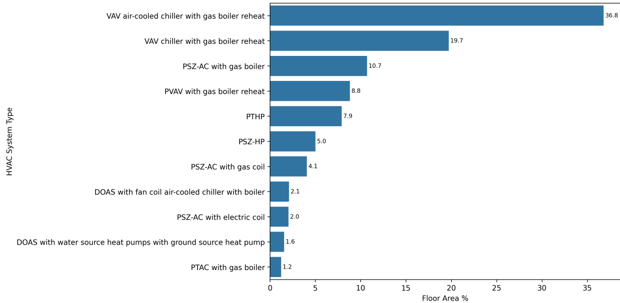
Figure 84. Prevalence of ComStock HVAC system types by total stock floor area; secondary schools.
